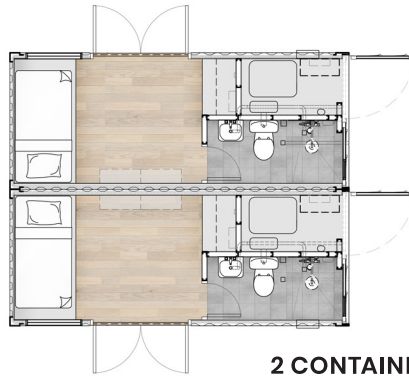
2 CONTAINER CONFIGURATION
